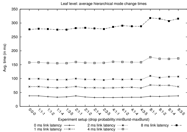
Figure 7. Hierarchical mode change operations at the leaf level in the management hierarchy.
