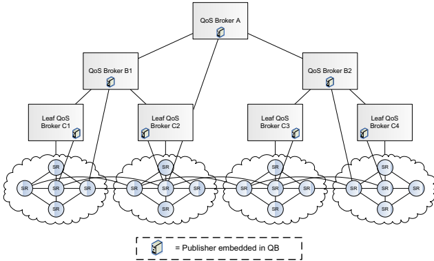
Figure 5. GridStat experimental setup - flood algorithm.
