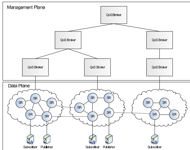
Figure 1. Status dissemination architecture
