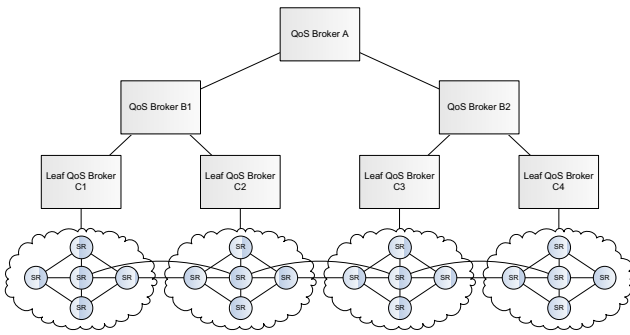
Figure 4. GridStat experimental setup - hierarchical algorithm.
